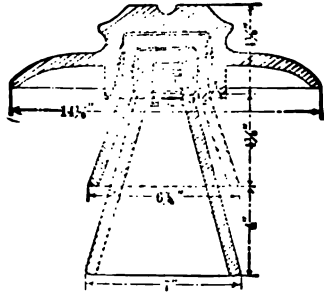
FIG. 16.—SECTION OF HIGH-TENSION INSULATOR.
